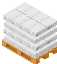
1 x 80X120 cm PALLET Qt. 13 levels (h 183.5 cm) Qt. 78 boxes Qt. 10,920 Chocup® Minis
